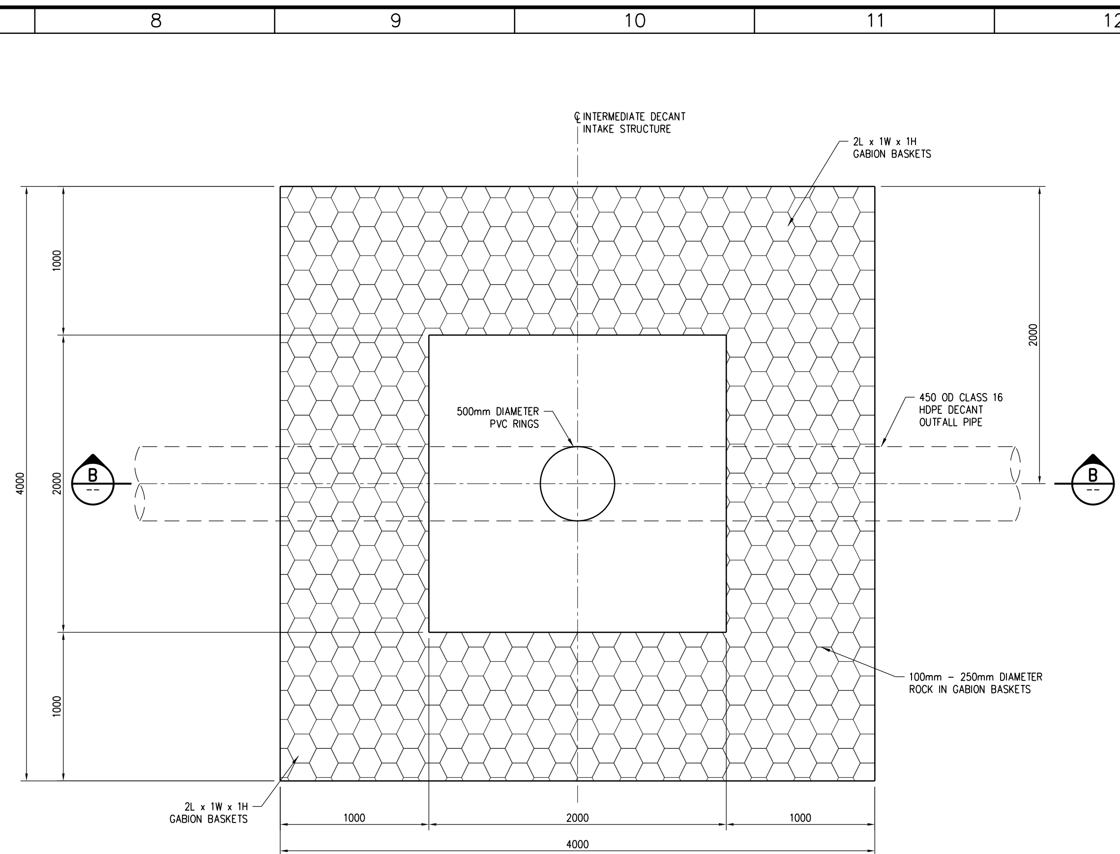
PLAN - INTERMEDIATE DECANT INTAKE STRUCTURE SCALE 1:25
