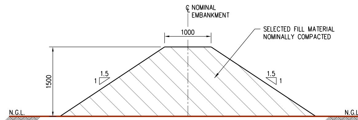
TYPICAL SECTION - NOMINAL EMBANKMENT SCALE 1:50
