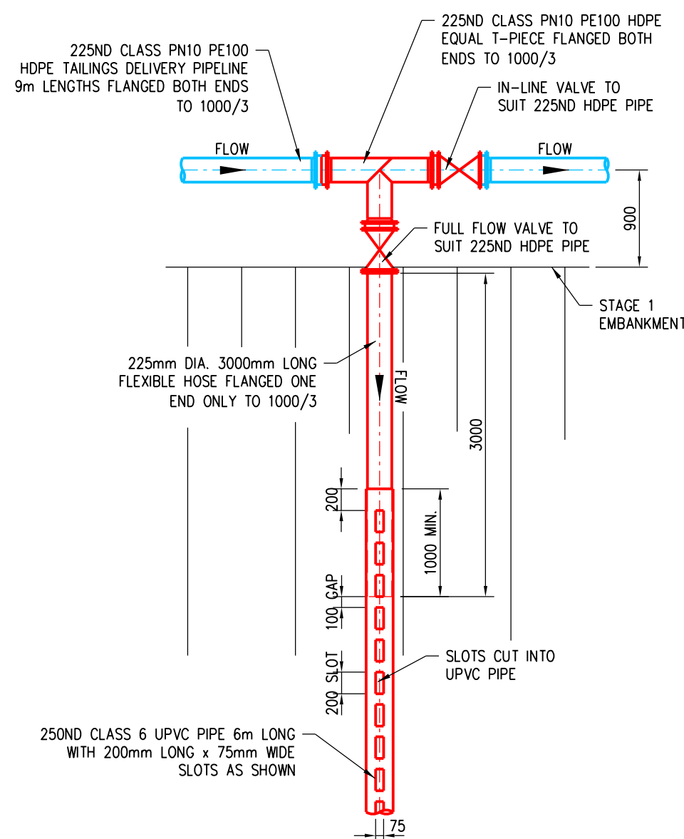
DETAIL 2 - PLAN FULL FLOW OUTLET 2 No. REQUIRED SCALE 1:50
