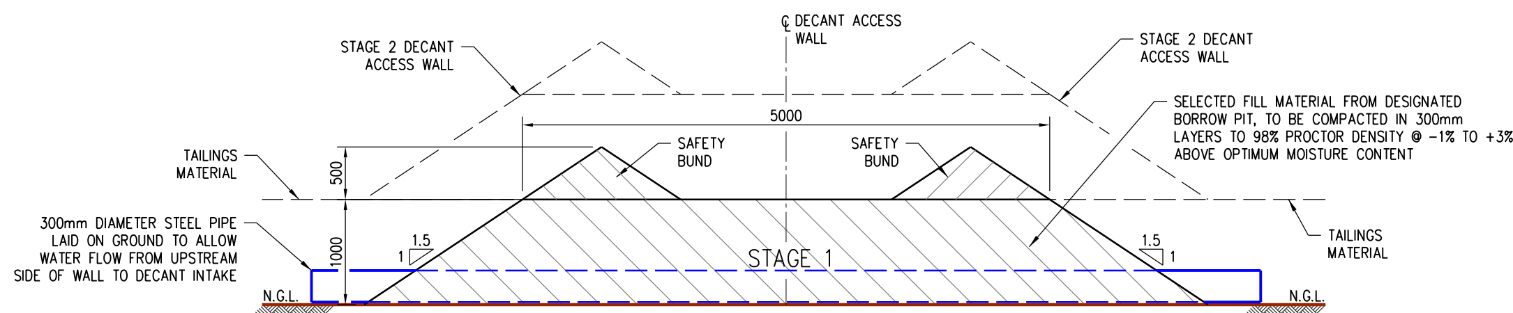
TYPICAL SECTION - DECANT ACCESS WALL SCALE 1:50
