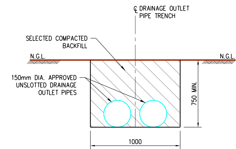
TYPICAL SECTION – DRAINAGE OUTLET PIPES SCALE 1:25
