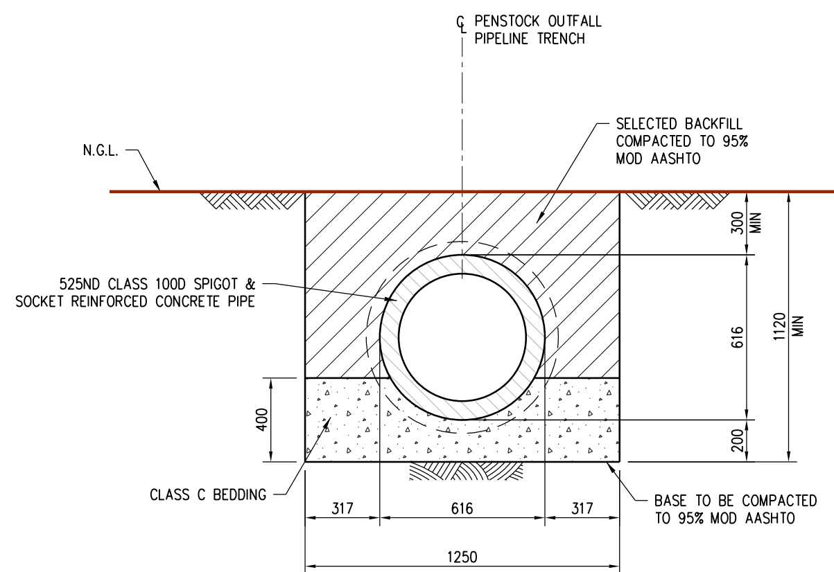
SECTION – PENSTOCK PIPE ON CLASS C BEDDING SCALE 1:25
