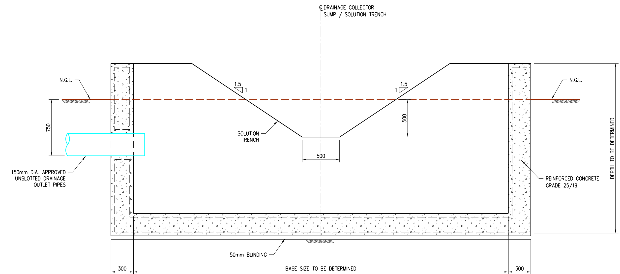
TYPICAL SECTION – DRAINAGE COLLECTOR SUMP SCALE 1:25
