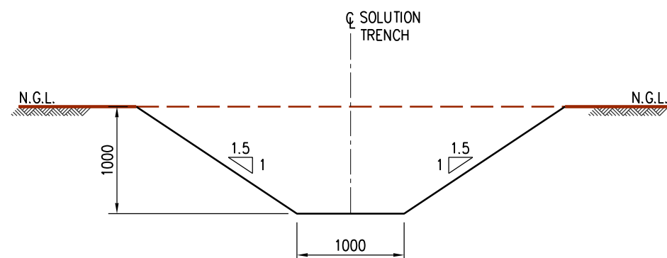
TYPICAL SECTION - SOLUTION TRENCH SCALE 1:50
