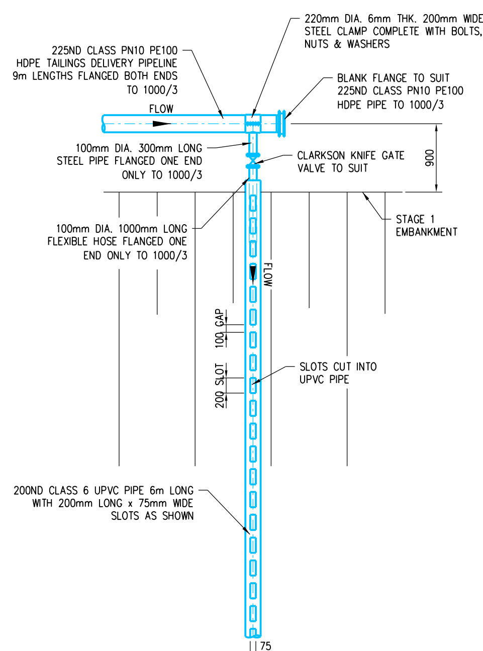
DETAIL 3 - PLAN SPIGOT OFF-TAKE AT PIPE END - 2 No. REQUIRED SCALE 1:50
