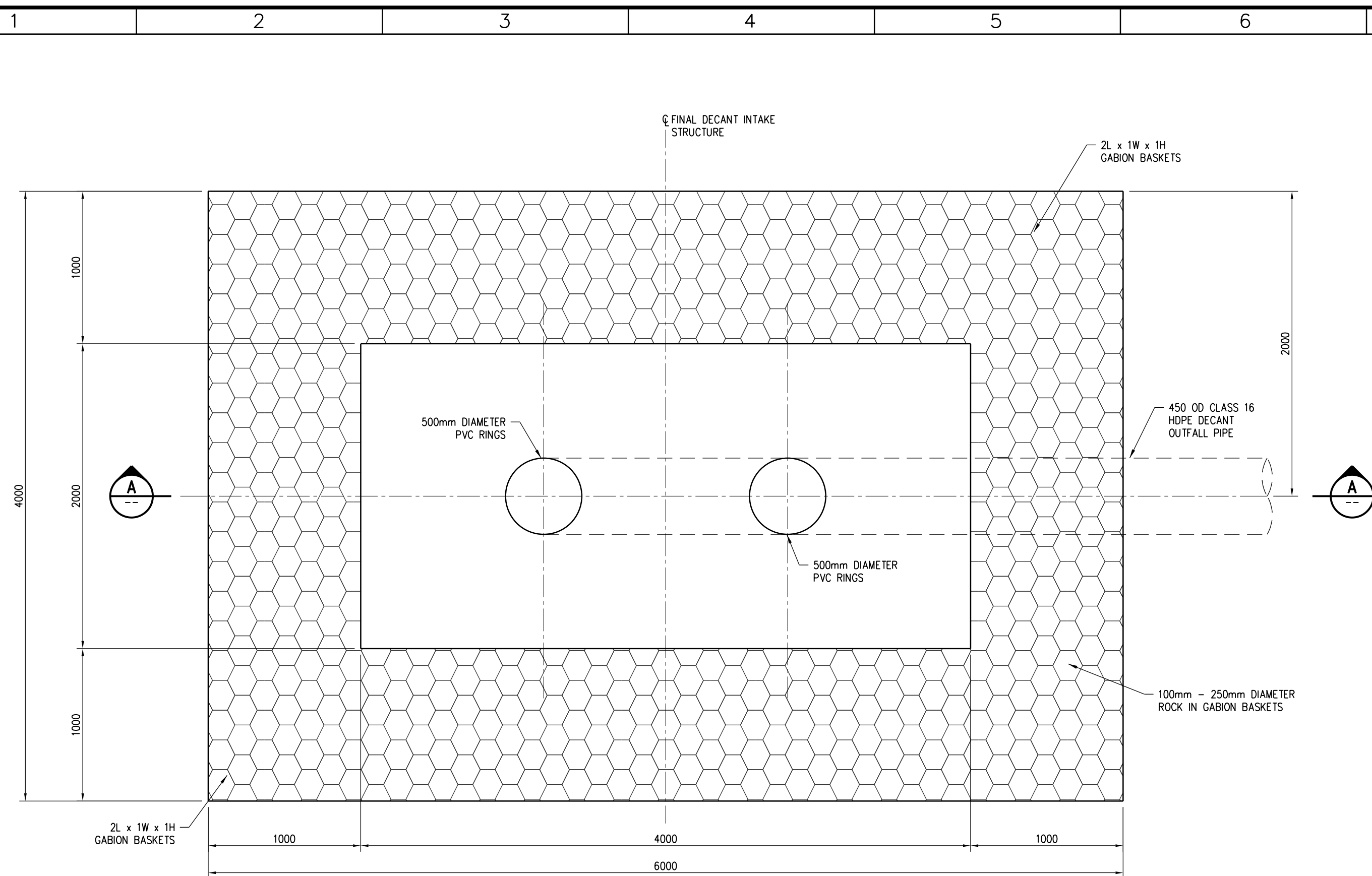
PLAN - FINAL DECANT INTAKE STRUCTURE SCALE 1:25
