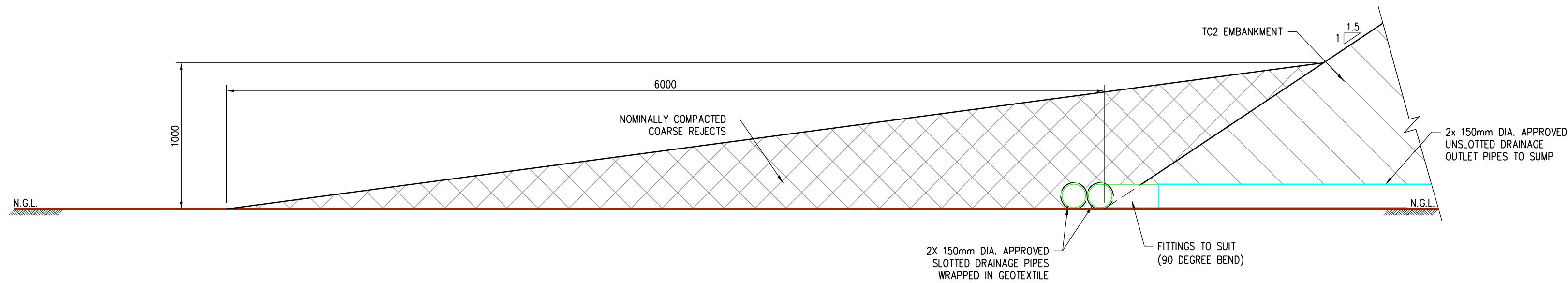
TYPICAL SECTION – HEEL DRAIN SCALE 1:25
