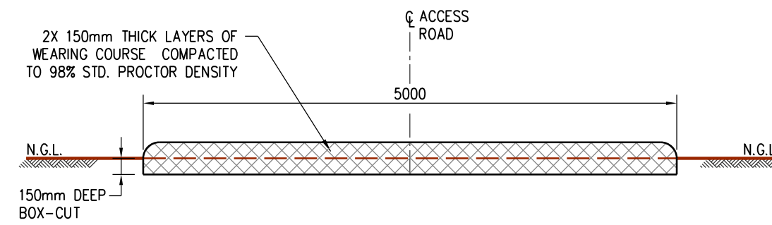
TYPICAL SECTION - ACCESS ROAD SCALE 1:50
