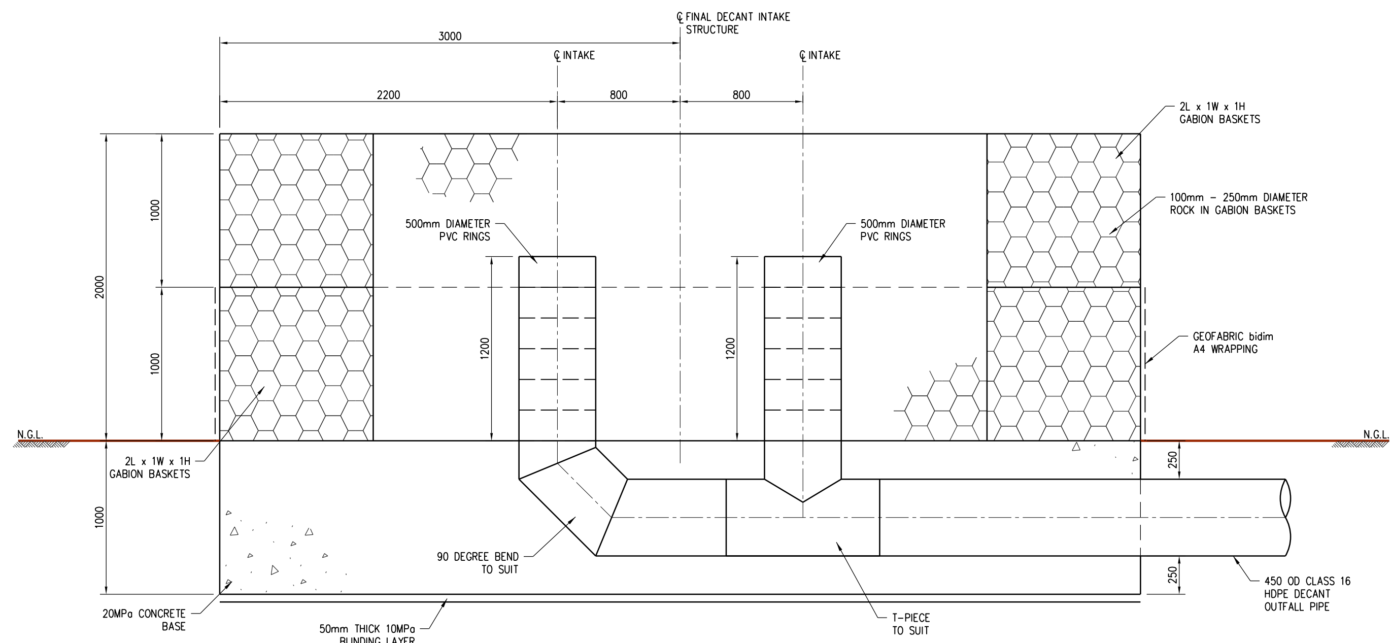
SECTION A 1:25
