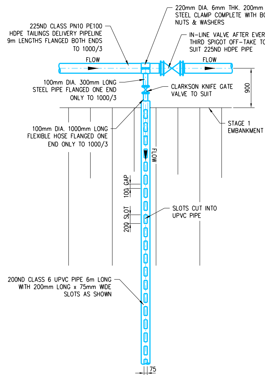
DETAIL 1 - PLAN SPIGOT OFF-TAKE 20 No. REQUIRED SCALE 1:50
